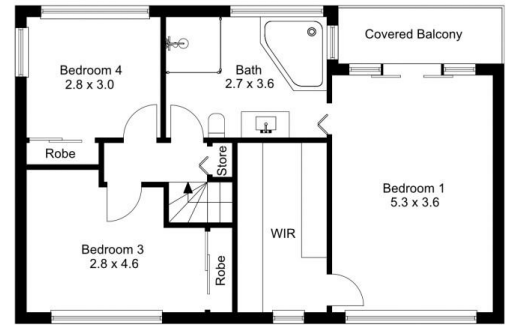
1st Floor
