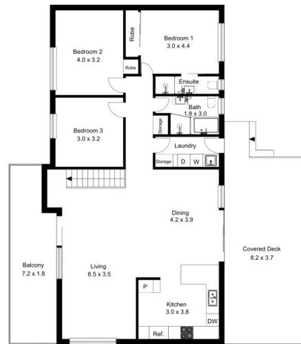
Upper Level
